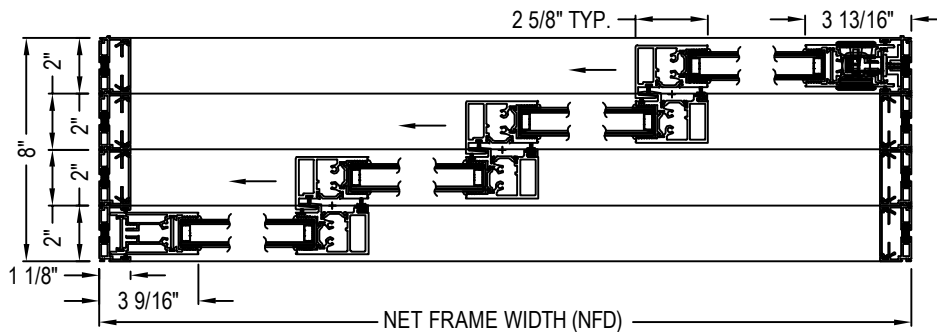
CROSS SECTION A-A: JAMBS
