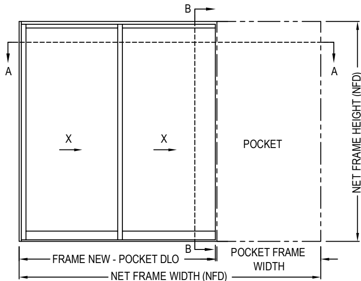
PLAN VIEW (SEEN FROM THE EXTERIOR)
