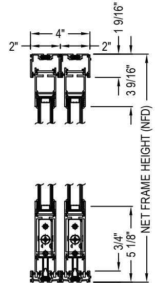
CROSS SECTION B-B: HEAD / THRESHOLD W/ 2" ULTRAGLIDE ROLLERS
