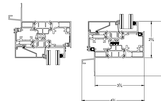
ASSEMBLY DRAWINGS
