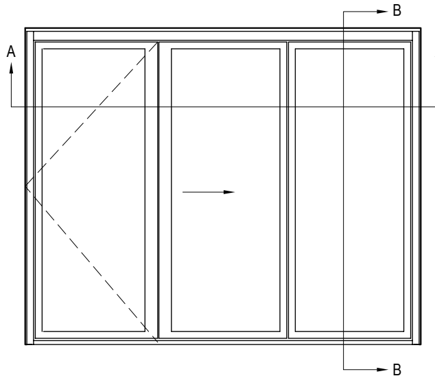
EXTERIOR ELEVATION
