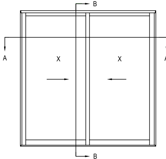
ELEVATION INTERIOR
