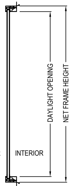
SECTION B-B
