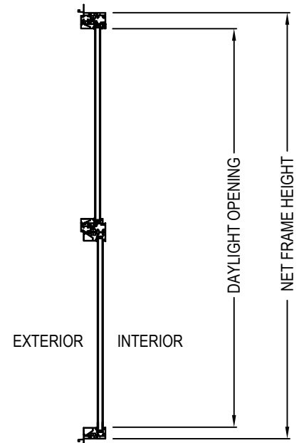
DETAIL B-B
