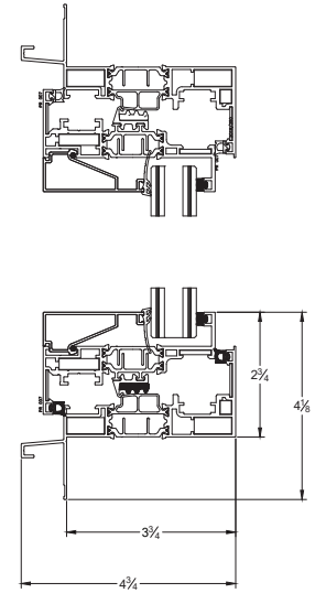
Assembly Drawings
