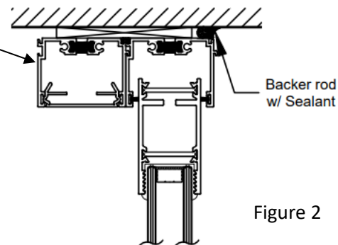
Head Part #14
